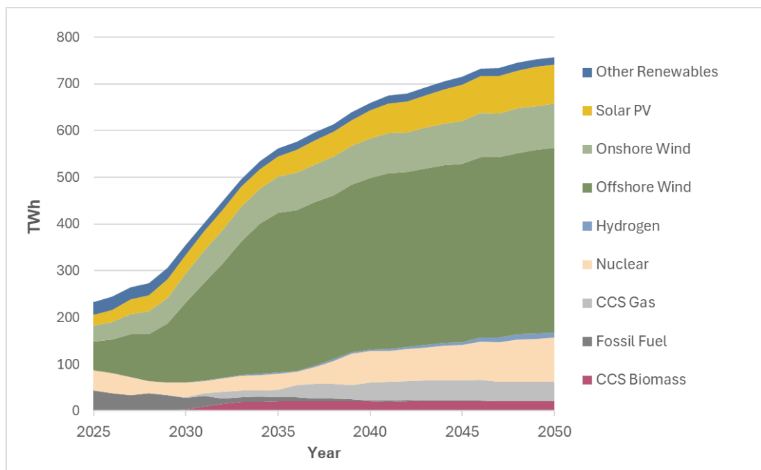
Figure 13-3: Electricity generation output by technology in Holistic Transition [Ref. 13-5327]
